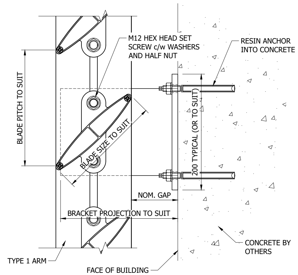
CLIMATE FACADE (TYPE 1 ARM) TO CONCRETE FACE FIX DETAIL
