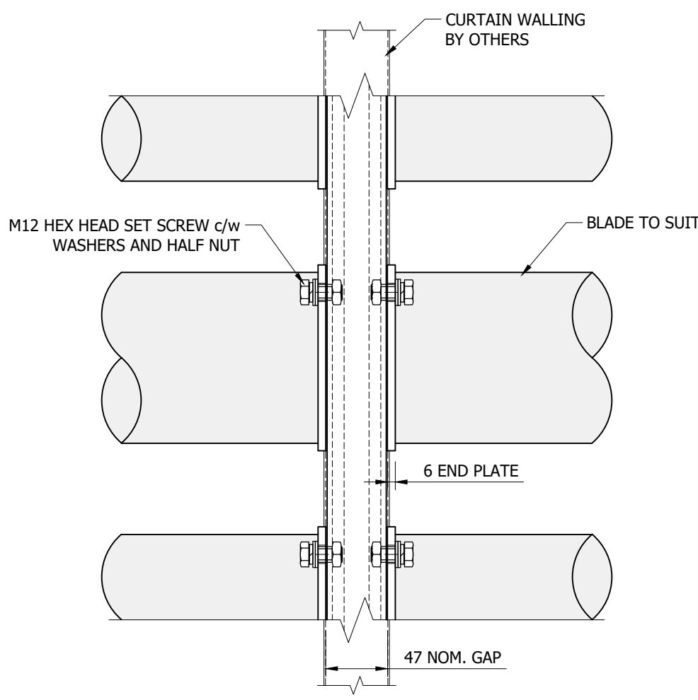
CLIMATE FACADE (TYPE 1 ARM) TO CURTAIN WALLING FIXING DETAIL
