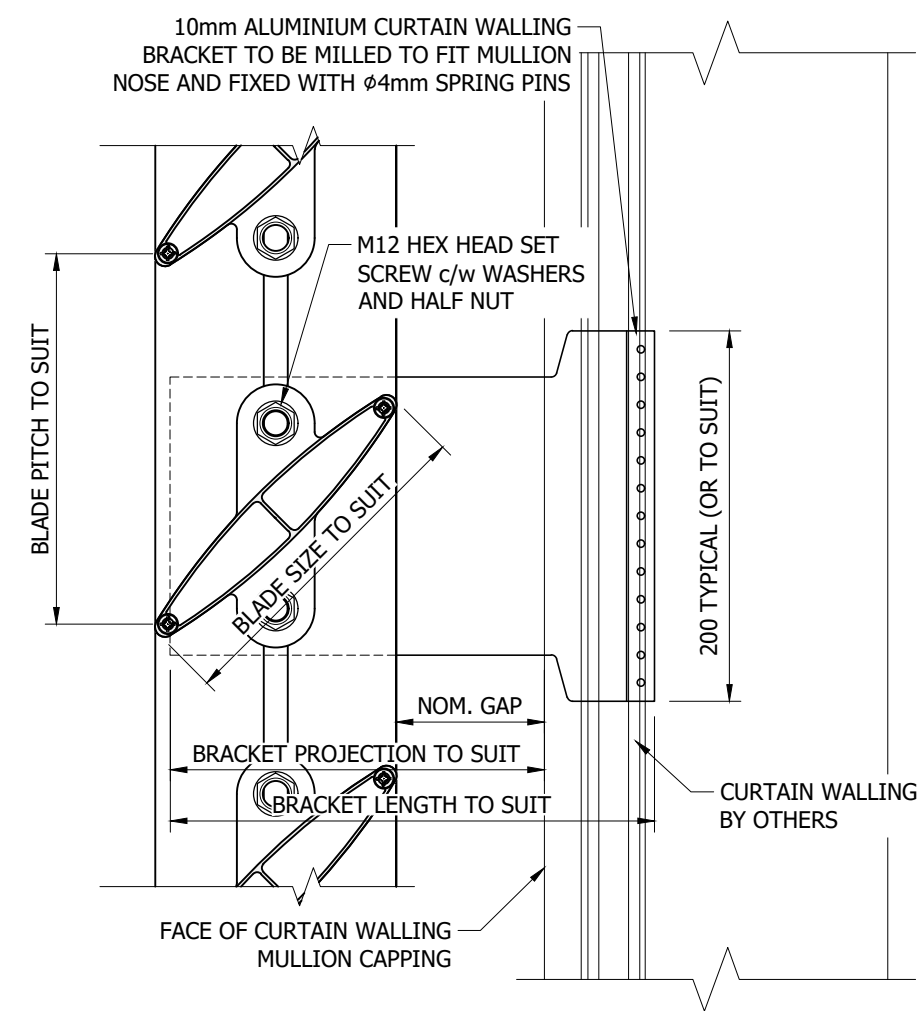
CLIMATE FACADE (TYPE 1 ARM) TO CURTAIN WALLING FIXING DETAIL
