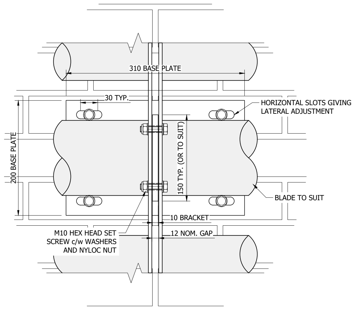
CLIMATE FACADE (CASSETTE) TO BRICKWORK FIXING DETAIL
